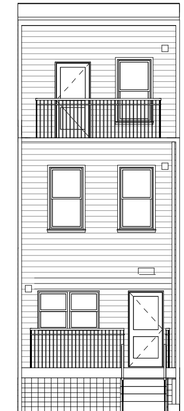
REAR ELEVATION - OPTION 1 & 2 (OPTIONAL DECK, DEPENDING ON GRADE)
